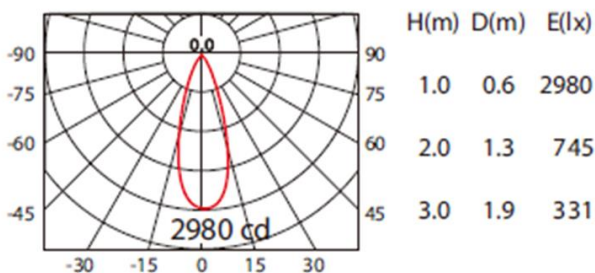
CoB 1500lm 350mA WW 36°
